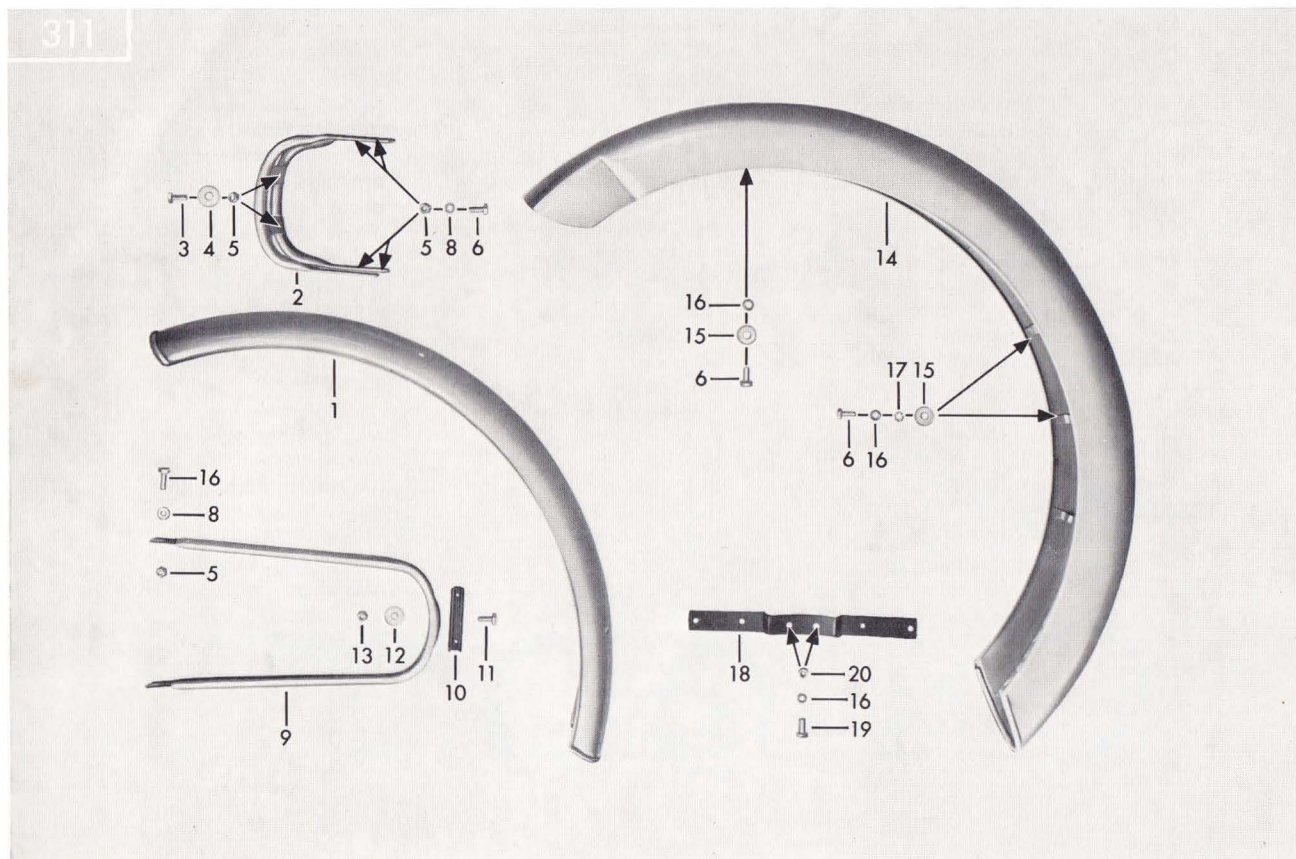
Tafel 16/1 Schutzbleche, Haltebügel, Nummernschildhalter Table 16/1 Fairings, mounting bracket, number plate bracket Planche 16/1 Garde-boue, étrier de retenue, support de plaque de police
