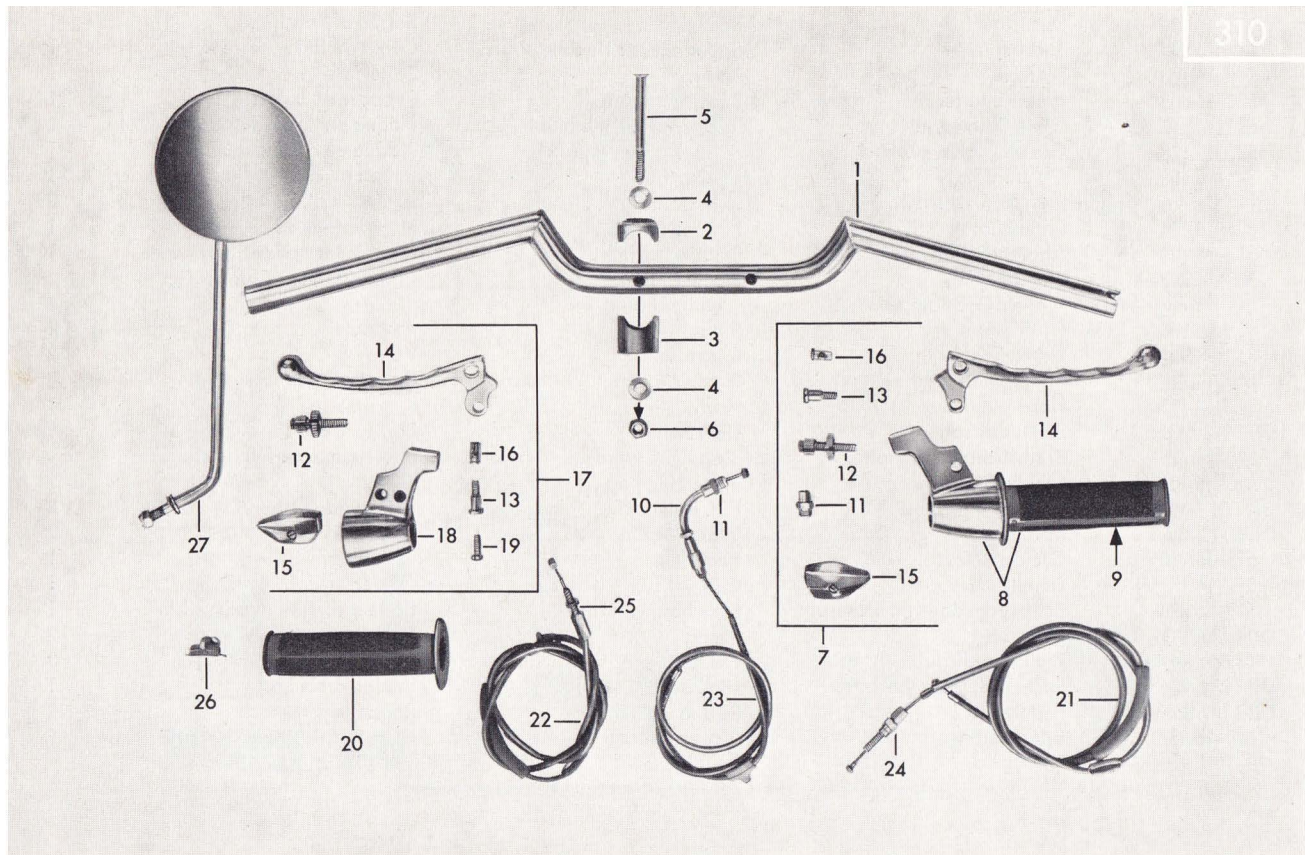
Tafel 15/1 Lenker, Armaturen, Seilzüge, Spiegel Table 15/1 Handlebar, operating levers and controls, cables, mirror Planche 15/1 Guidon, leviers et tirettes de commande, câbles, miroir
