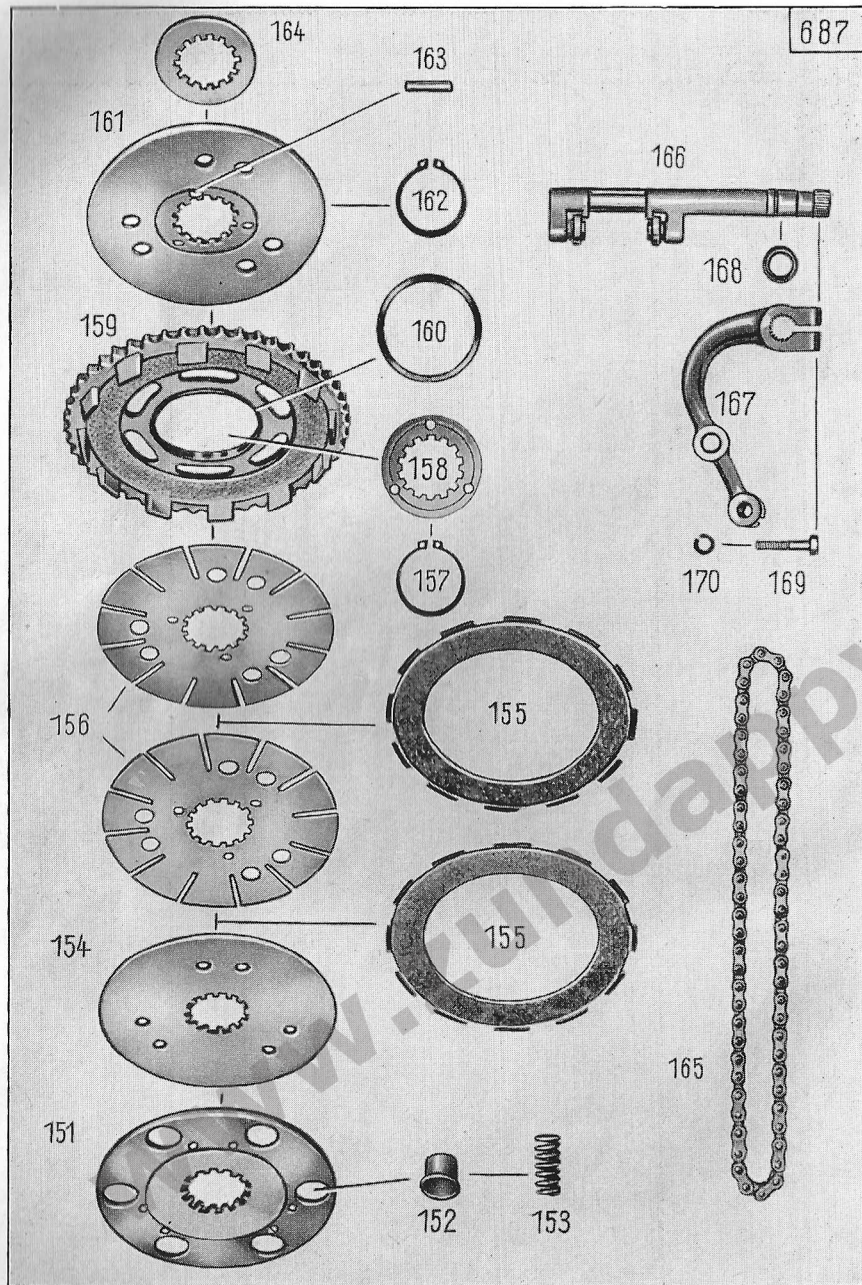
Illustration 8, Group M: g) Clutch, clutch, operating mechanism
