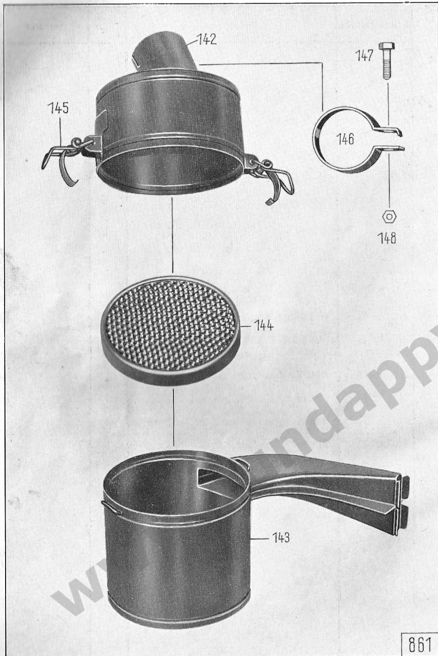
Illustration 7, Group M: f) Carburettor Intake Silencer
