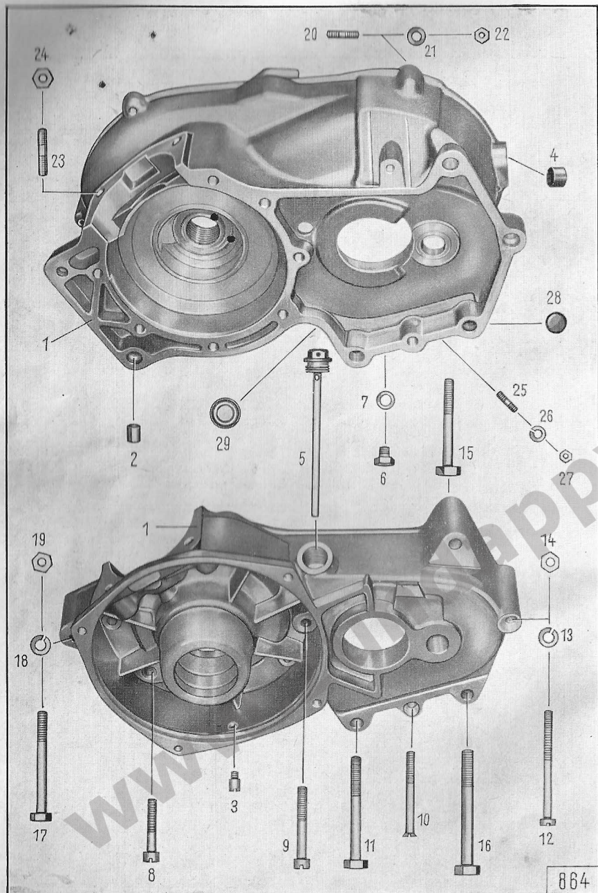
Illustration 2, Group M: Housing and Cylinder, Crankcase
